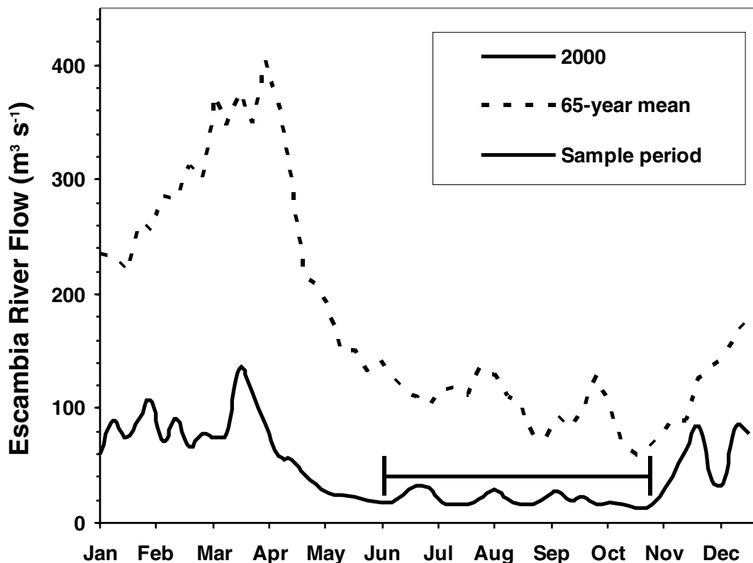
Figure 3. Hydrograph for the Escambia River discharge ( \text{m}^3 \text{s}^{-1} ). The solid line shows the discharge from 2000, whereas the dashed line shows the historical mean weekly flow averages. The horizontal bar indicates the period during which benthic flux studies occurred.
